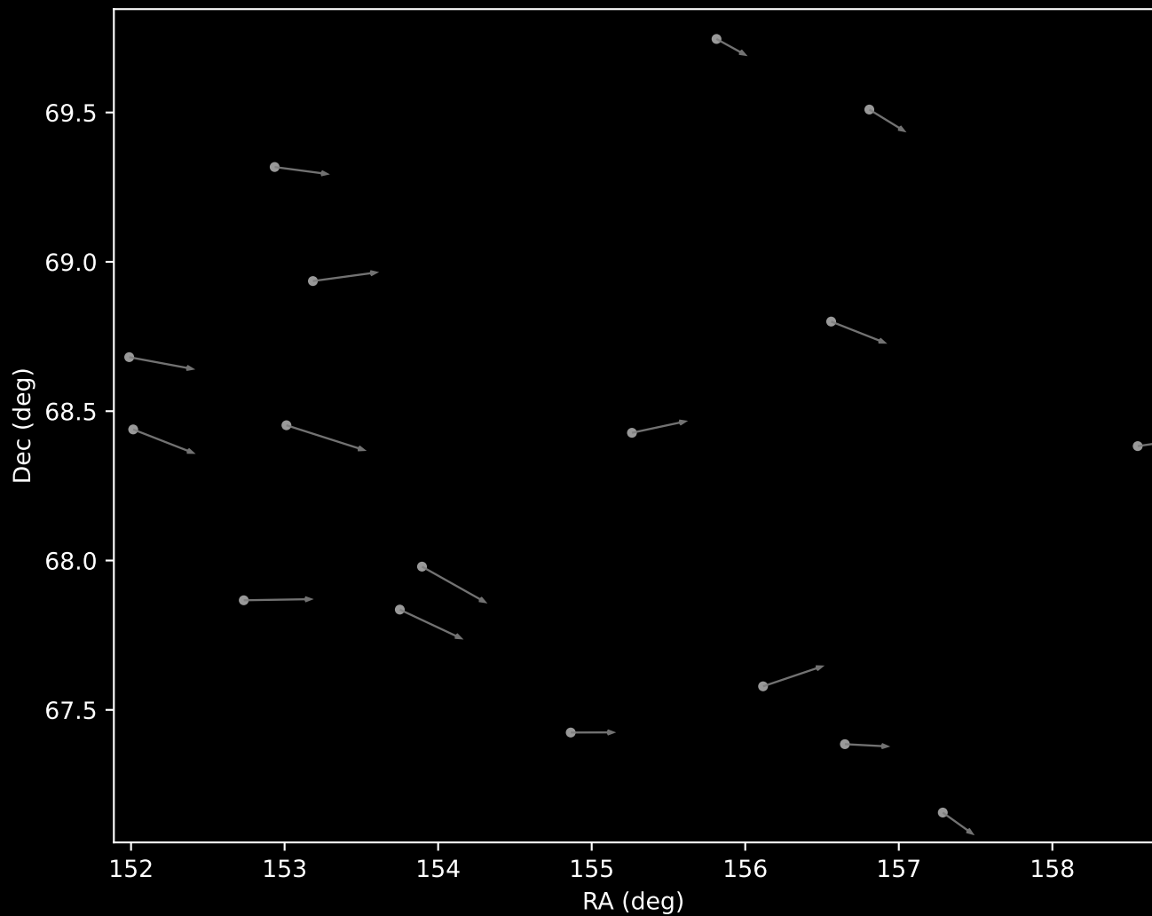
APOGEE DR17 Cluster 74 Proper Motion Vectors (n=17)
