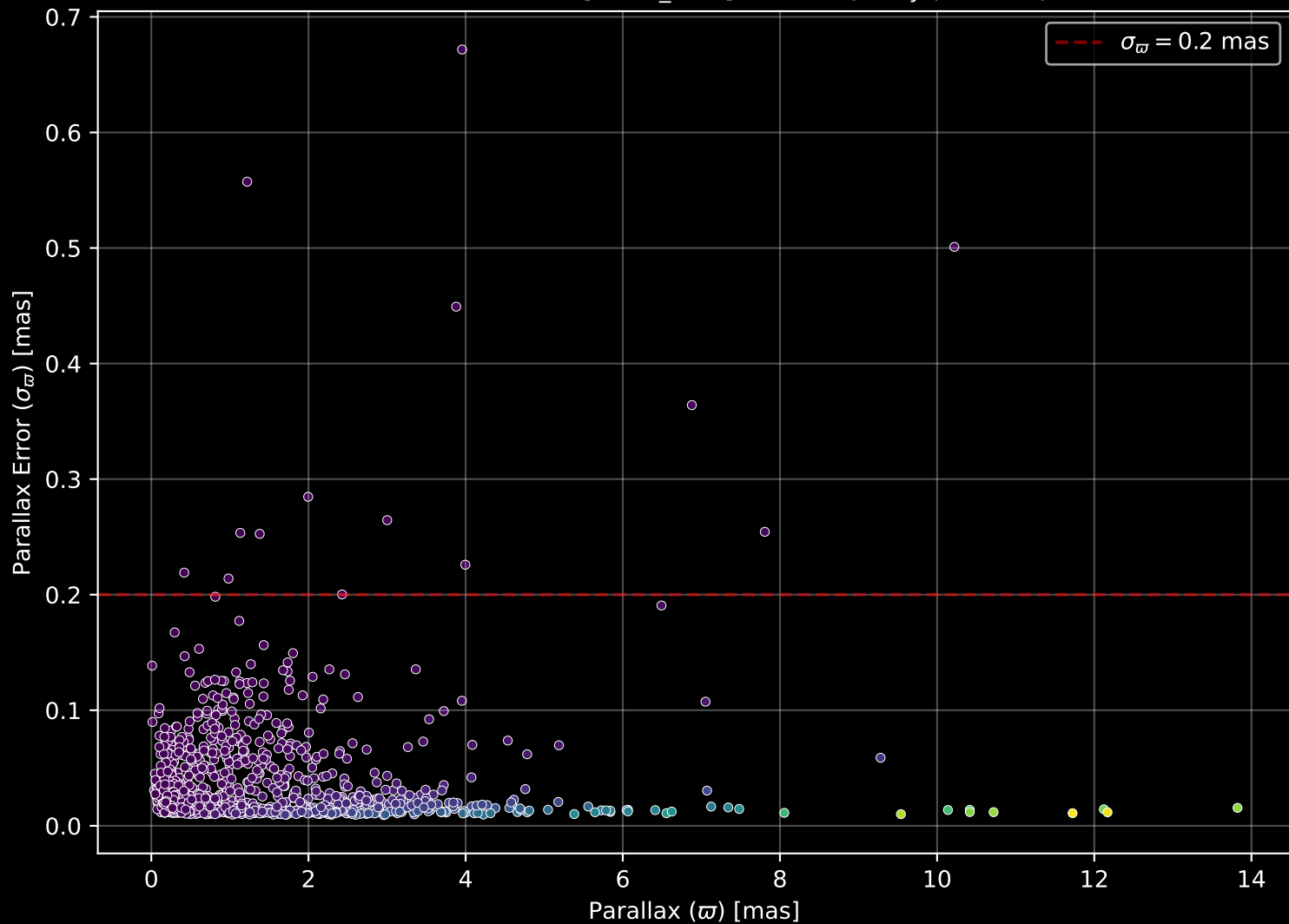
APOGEE DR17 Field: [IC342_MGA] Parallax Quality (n= 1659)
