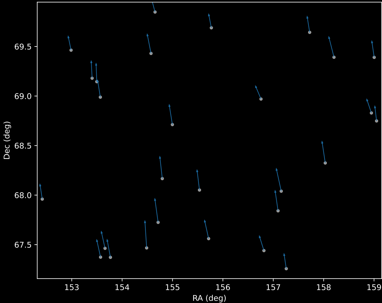
APOGEE DR17 Cluster 60 Proper Motion Vectors (n=28)
