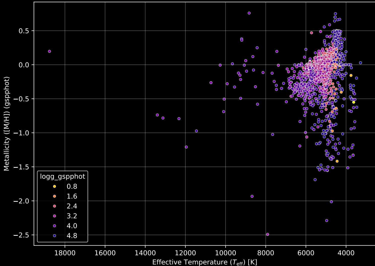
APOGEE DR17 Field: [IC342_MGA] Stellar Population Parameters (n= 1659)
