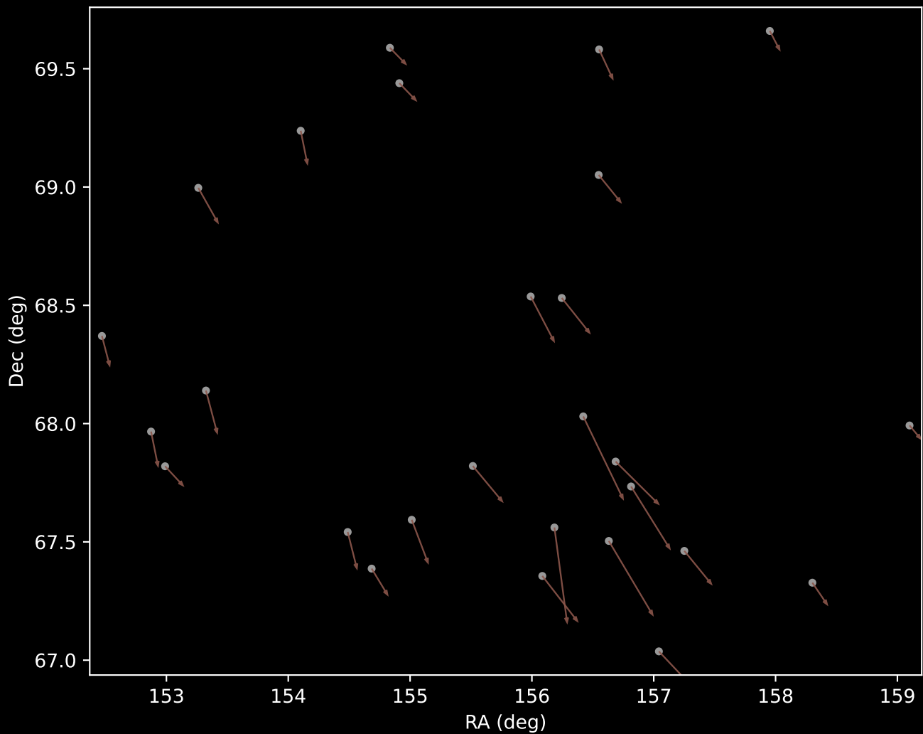
APOGEE DR17 Cluster 70 Proper Motion Vectors (n=27)
