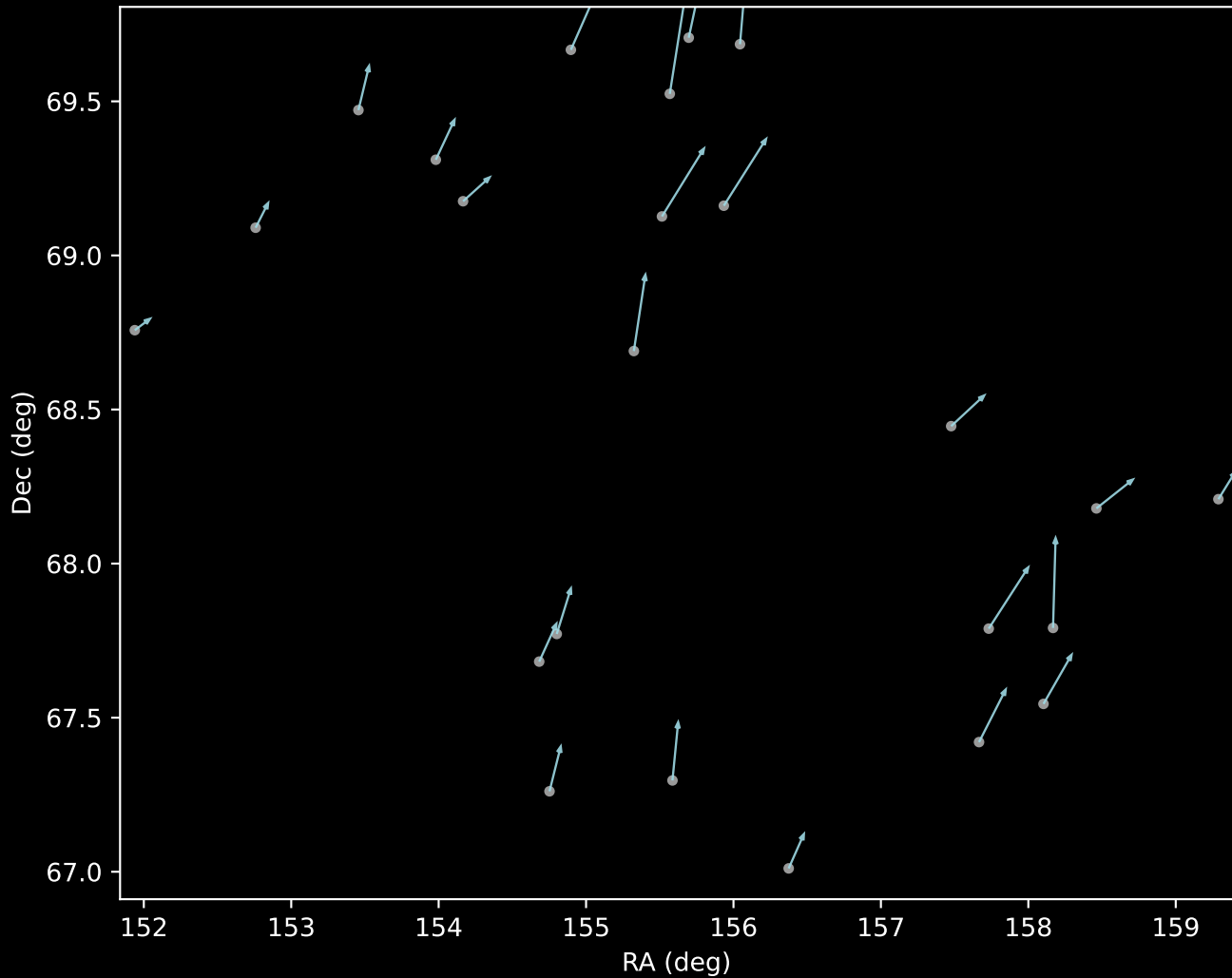
APOGEE DR17 Cluster 79 Proper Motion Vectors (n=24)
