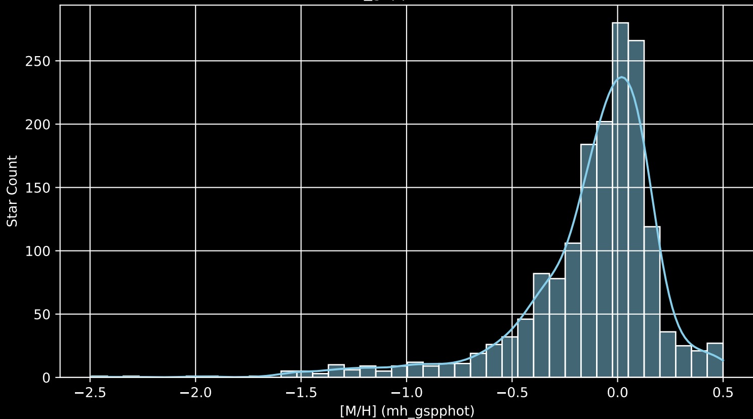
APOGEE DR17 Field: [IC342_MGA [M/H] (mh_gspphot) (n= 1649)
