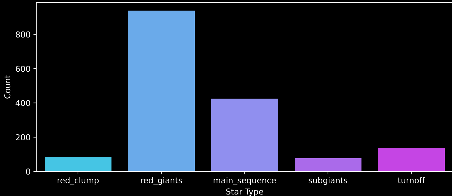
APOGEE DR17 Field: [IC342_MGA] Count plot of Star Type
