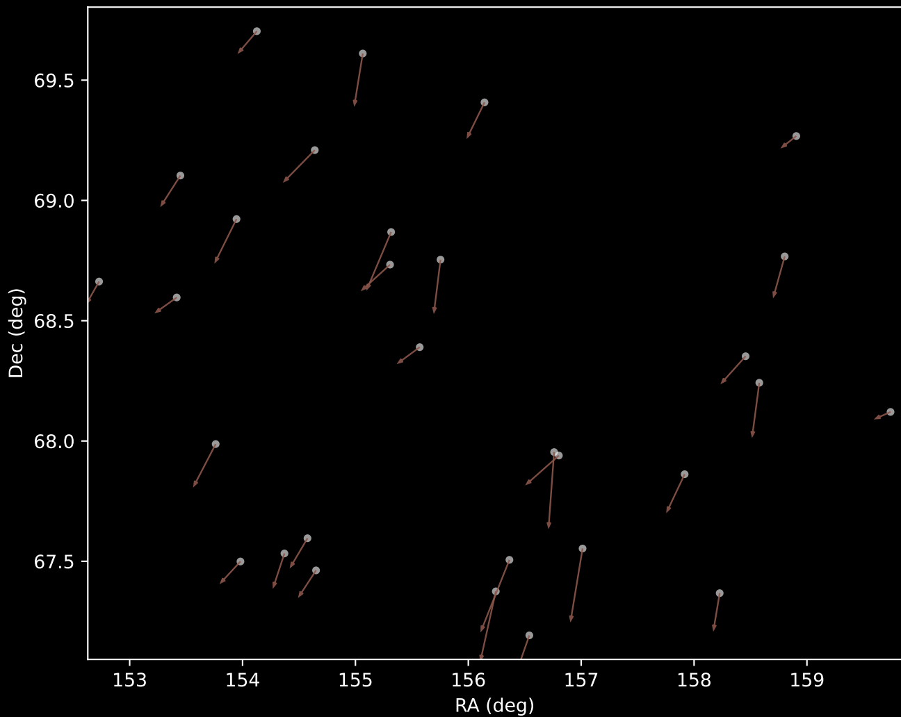
APOGEE DR17 Cluster 50 Proper Motion Vectors (n=30)
