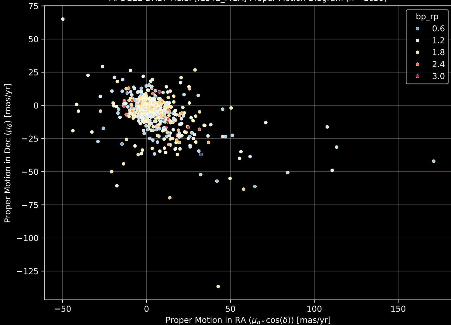
APOGEE DR17 Field: [IC342_MGA] Proper Motion Diagram (n= 1659)
