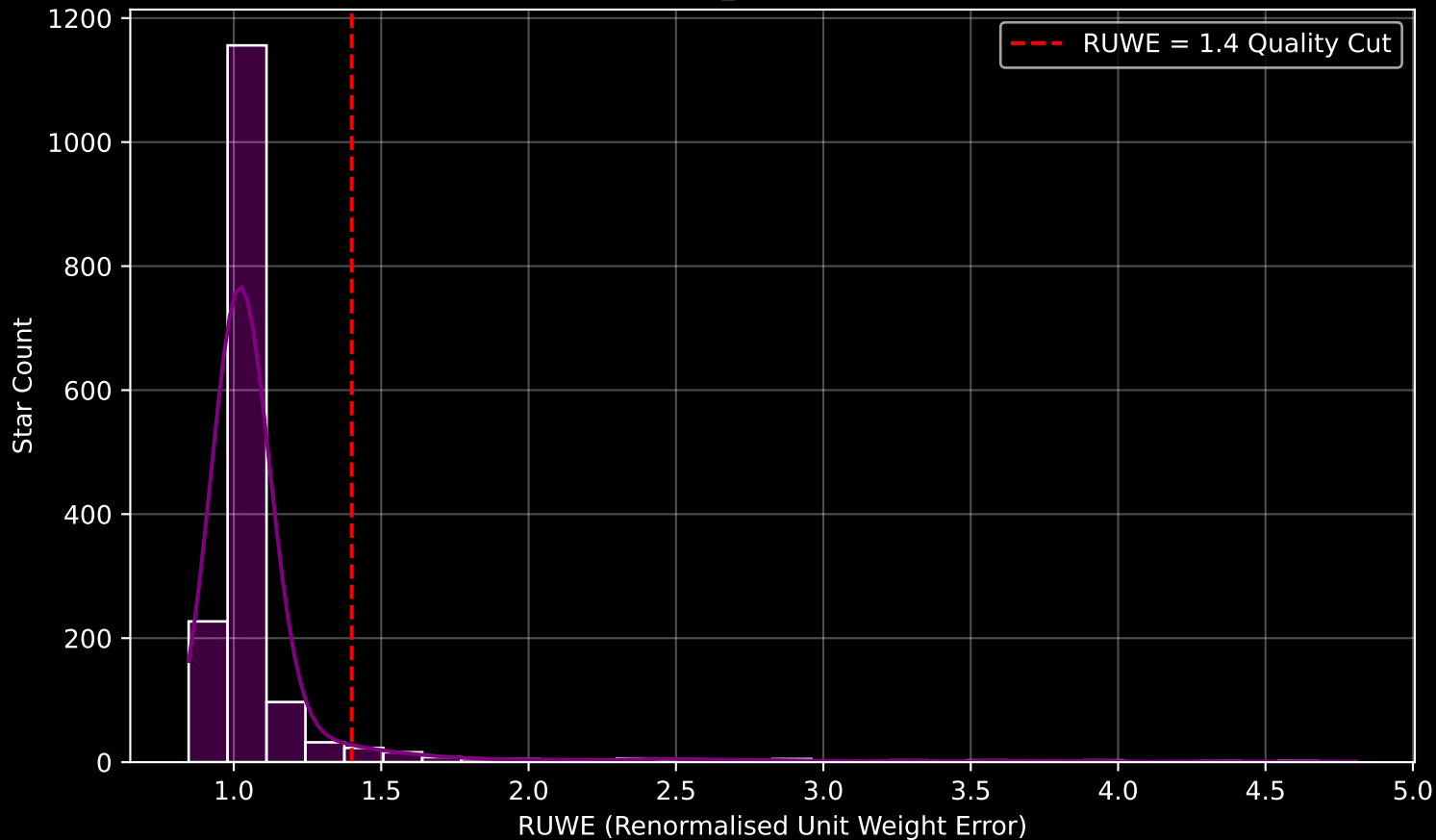
GAPOGEE DR17 Field [IC342_MGA] RUWE Distribution (n= 1617)
