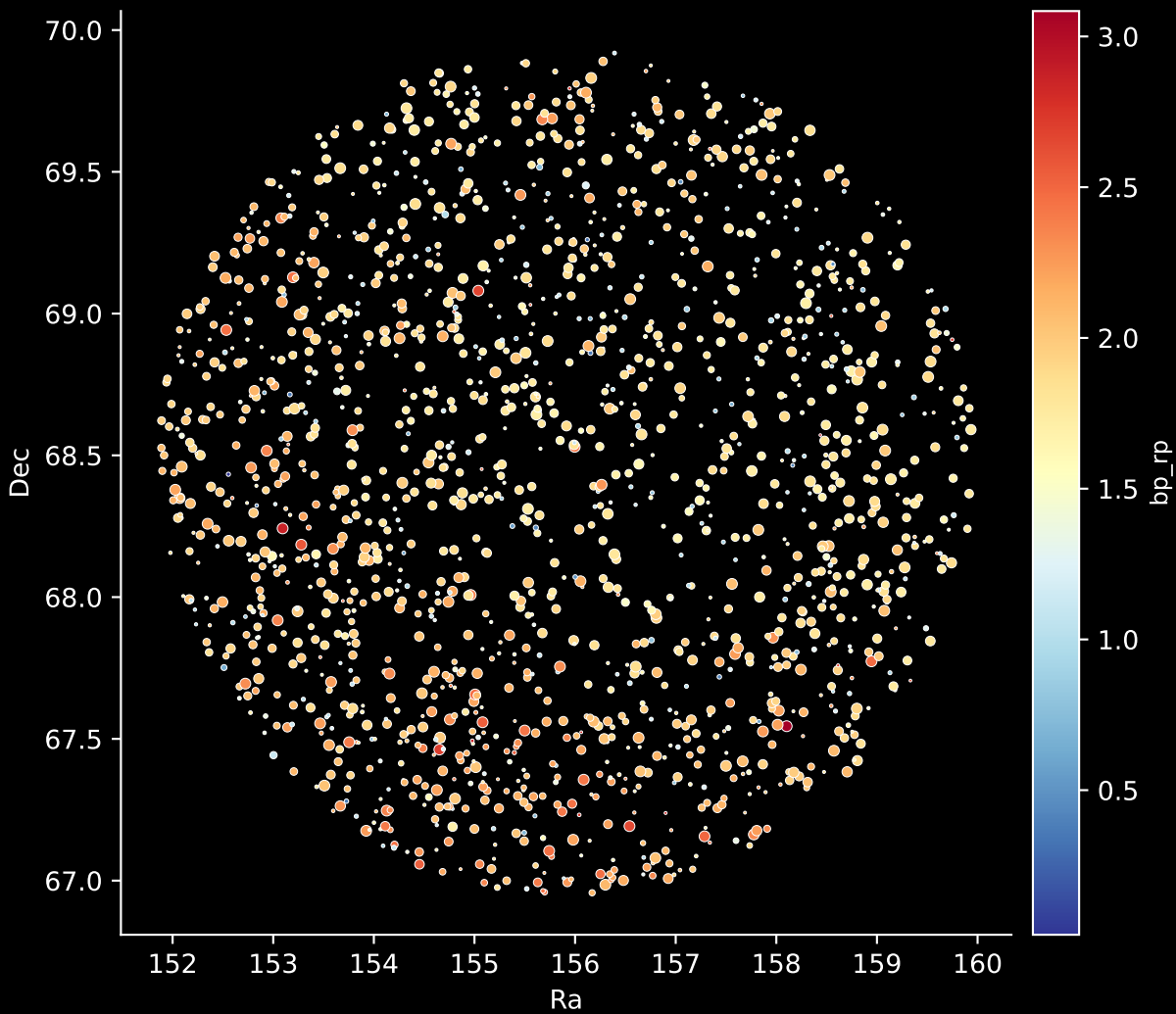
APOGEE DR17 Field: [IC342_MGA] Stars: 1659
