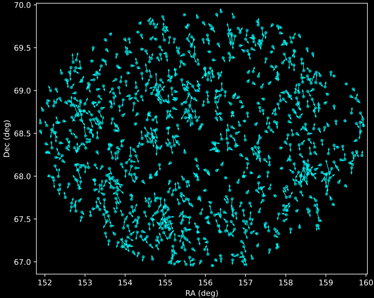
APOGEE DR17 Noise Stream Proper Motion Vectors (n=886)
